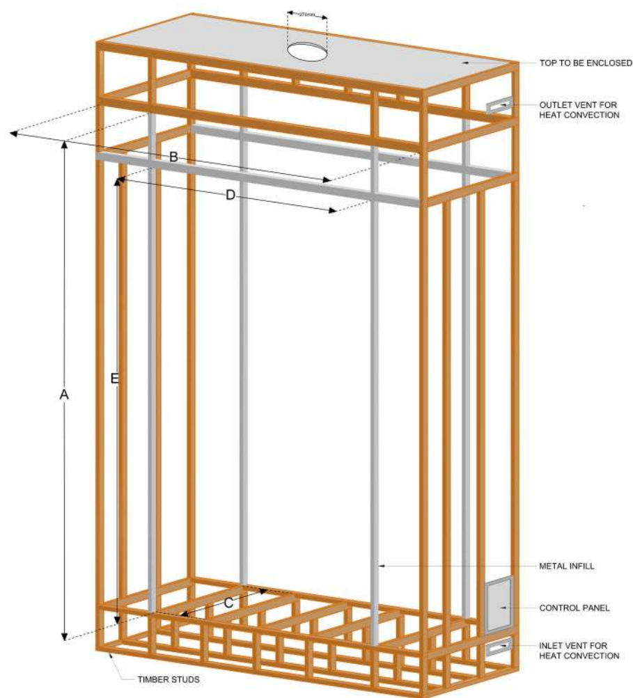
Figure 1.8 (Timber framing)
